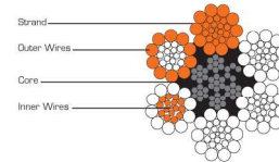
Rope End View
